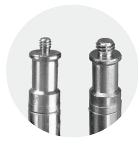
1/4" and 3/8" stud at the end of arm.
